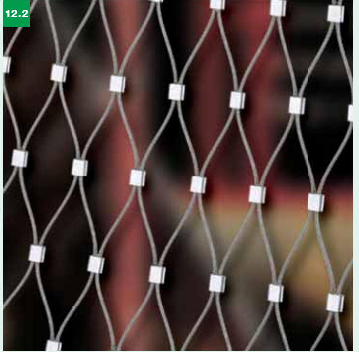
Webnet with 35° mesh angle
