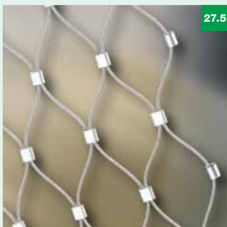
Vertical mesh perimeter: with uncompressed sleeves at right
