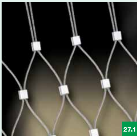
Vertical mesh perimeter: open at top with wire-rope end pairs
